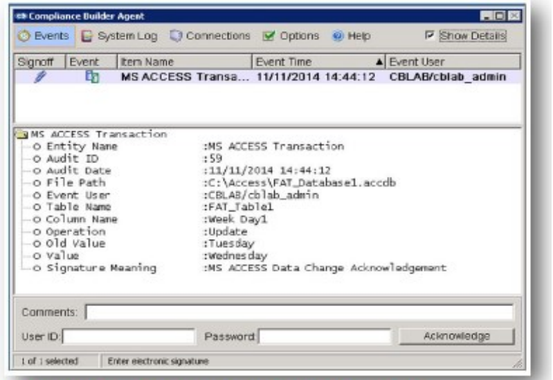
Figure 2. ComplianceBuilder supports flexible transaction monitoring on databases, including Microsoft Access.
